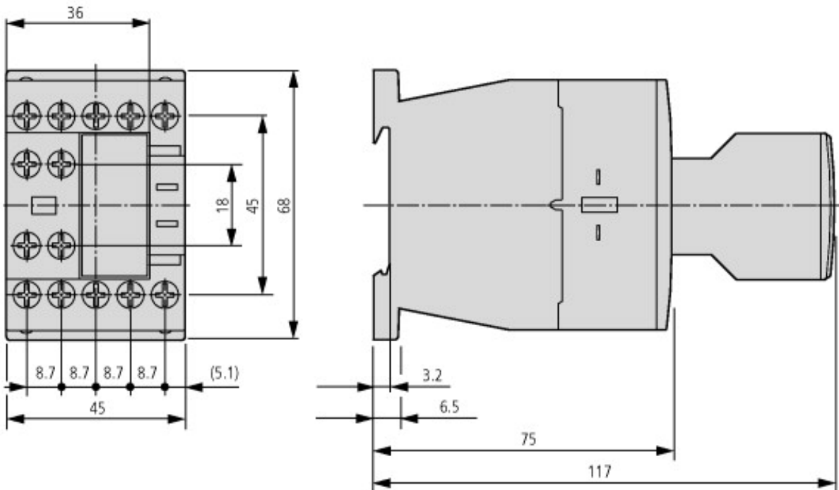
Contactors with auxiliary contact module DILM32-XHI.../DILA-XHI...
